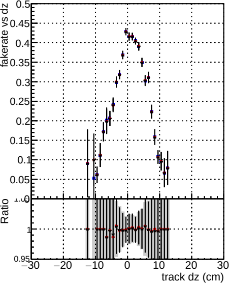
Fake rate vs dz Legend: DOM TT original_lowpt newbranch_lowpt newbranch_lowpt_pless newbranch_lowpt_pless_MVACand
