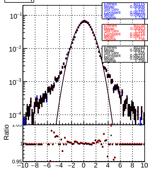
— BOM TT original lowpt — BOM TT newbranch lowpt — pLess — BOM TT newbranch lowpt pLessMVAand
