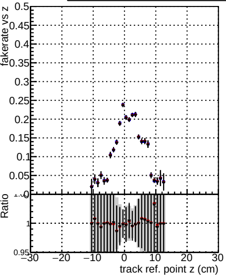
Fake rate vs vertpos —■— DQM TT original_lowpt —●— DQM TT newbranch_lowpt_pLess —▲— DQM TT newbranch_lowpt_pLessMVACand
