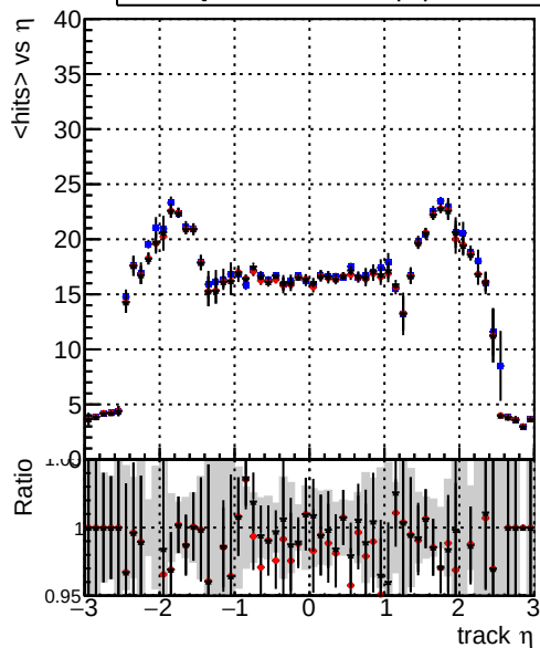
mean hits — DQM_TT_original_lowpt — DQM_TT_newbranch_lowpt_pLess — DQM_TT_newbranch_lowpt_pLessMVACand
