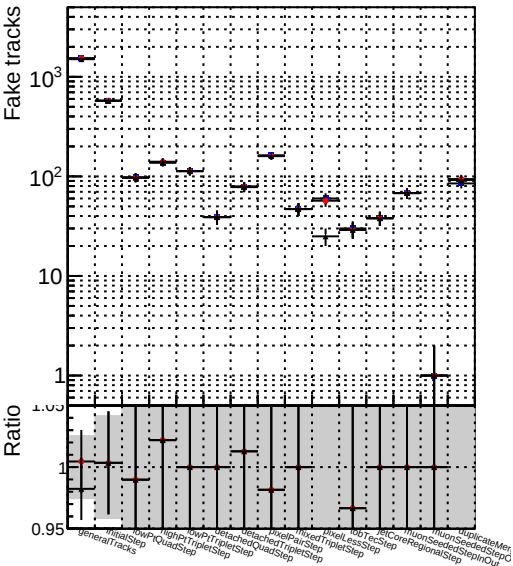
Number Legend ● DQM_TT_newbranch_lowpt_pLess ★ DQM_TT_newbranch_lowpt_pLessMVA Cand
