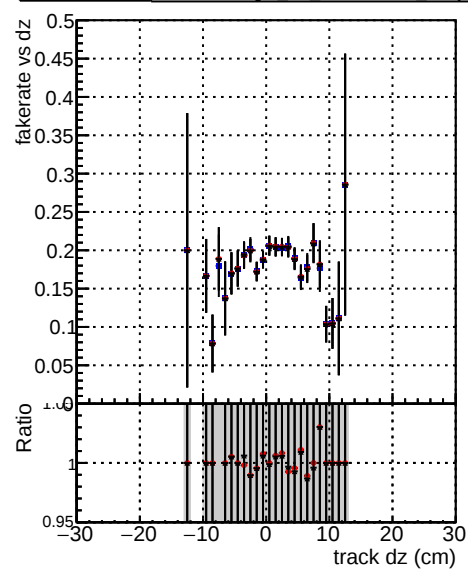
—•— DOM TT original_lowpt —•— DOM TT newbranch_lowpt_pLess —•— DOM TT newbranch_lowpt_pLess_MVACand
