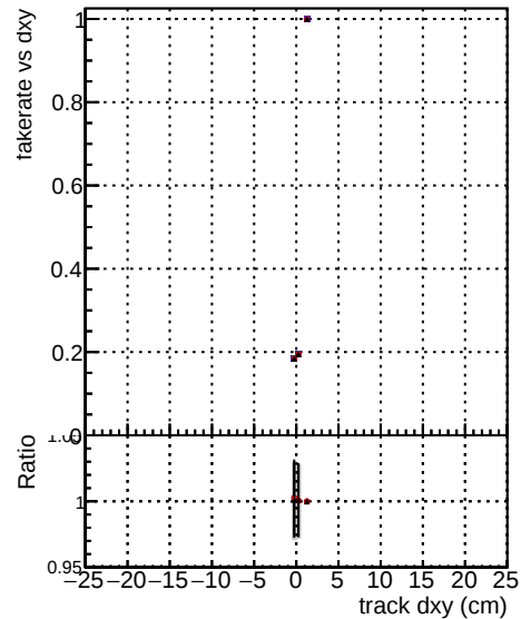
—•— DOM TT original_lowpt —•— DOM TT newbranch_lowpt_pLess —•— DOM TT newbranch_lowpt_pLess_MVACand
