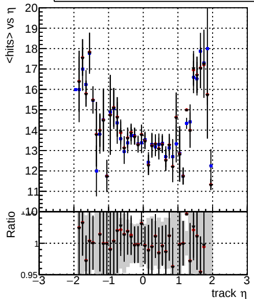
mean hit — DQM_TT_original_lowpt — DQM_TT_newbranch_lowpt_pLess — DQM_TT_newbranch_lowpt_pLessMVACand
