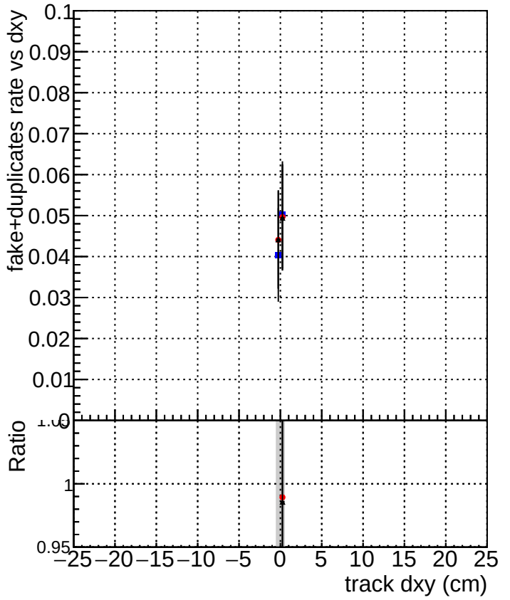
Legend for the bottom plot: DQM_TT_original_lowpt (blue square) DQM_TT_newbranch_lowpt_pLess (red circle) DQM_TT_newbranch_lowpt_pLessMVACand (black triangle)
