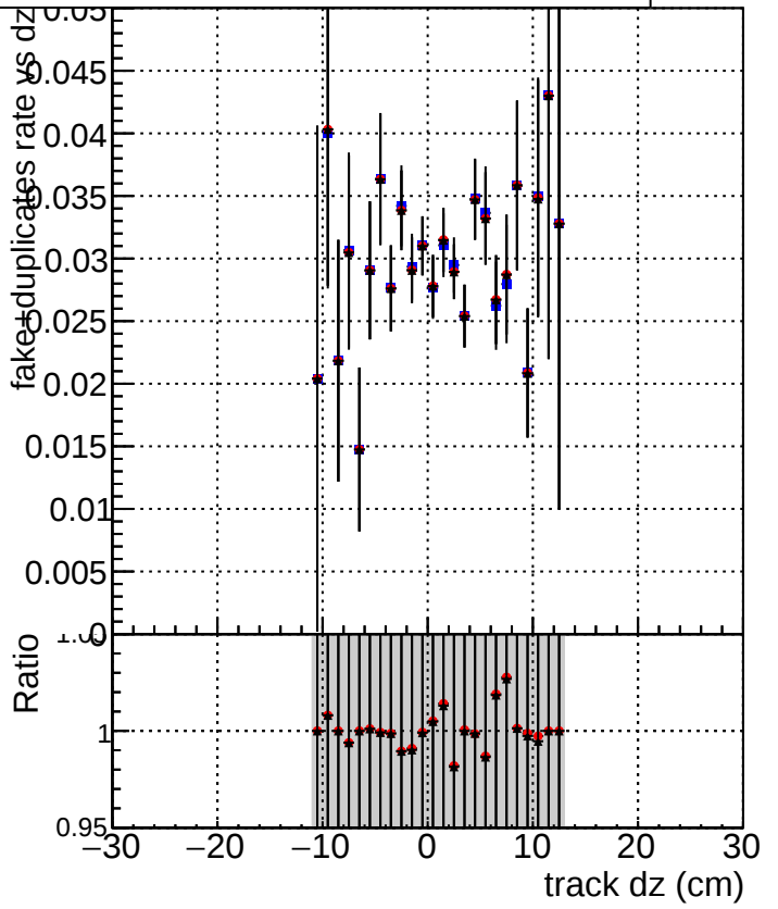
Legend: DQM_TT_original_lowpt DQM_TT_newbranch_lowpt_pLess DQM_TT_newbranch_lowpt_pLessMVAand
