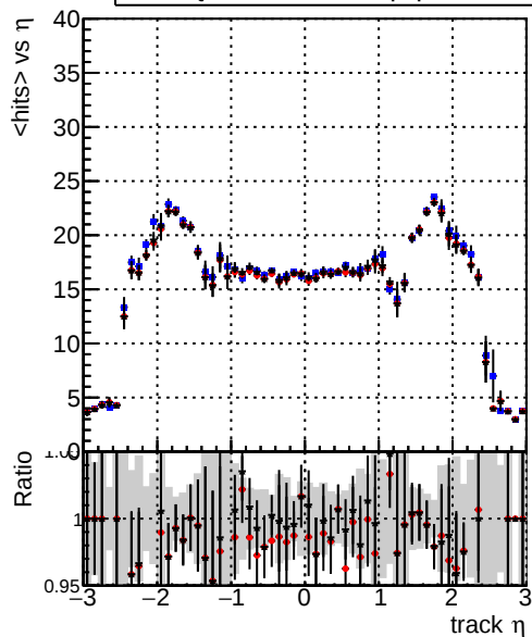
mean hits — DQM_TT_original_lowpt — DQM_TT_newbranch_lowpt_pLess — DQM_TT_newbranch_lowpt_pLessMVA
