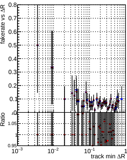
Fake rate vs \Delta R(\text{track, jet}) Legend: DQM TT original_lowpt (blue dots) DQM TT newbranch_lowpt_pLess (red dots) DQM TT newbranch_lowpt_pLessMVACand (black dots)
