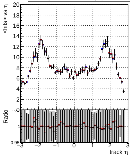
mean hit — DQM_TT_original_lowpt — DQM_TT_newbranch_lowpt_pLess — DQM_TT_newbranch_lowpt_pLessMVACand
