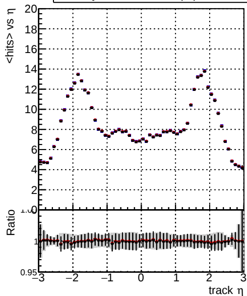
mean hits — DQM_TT_original_lowpT — DQM_TT_newbranch_lowpT_pLess — DQM_TT_newbranch_lowpT_pLessMVACand
