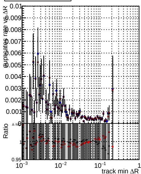
—•— DQM_TT_original_lowpt —•— DQM_TT_newbranch_lowpt_pLess —•— DQM_TT_newbranch_lowpt_pLessMVACand
