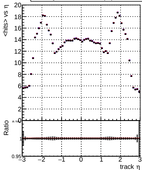
mean hits vs \eta — DQM_TT_original_lowpt — DQM_TT_newbranch_lowpt_pLess — DQM_TT_newbranch_lowpt_pLessMVACand
