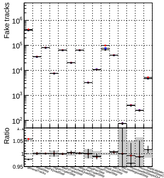
Number of tracks vs collection DQM_TT_original_lowpt DQM_TT_newbranch_lowpt_pLess DQM_TT_newbranch_lowpt_pLessMVACand
