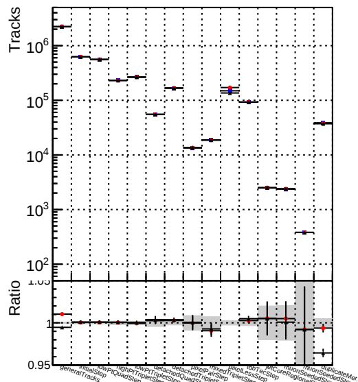
Number of tracks vs collection DQM_TT_original_lowpt DQM_TT_newbranch_lowpt_pLess DQM_TT_newbranch_lowpt_pLessMVACand
