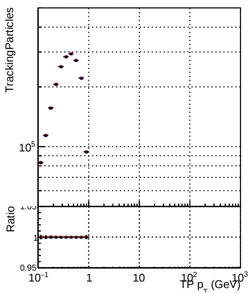
—•— DQM_TT_original_lowpt —•— DQM_TT_newbranch_lowpt_pLess —•— DQM_TT_newbranch_lowpt_pLessMVACand
