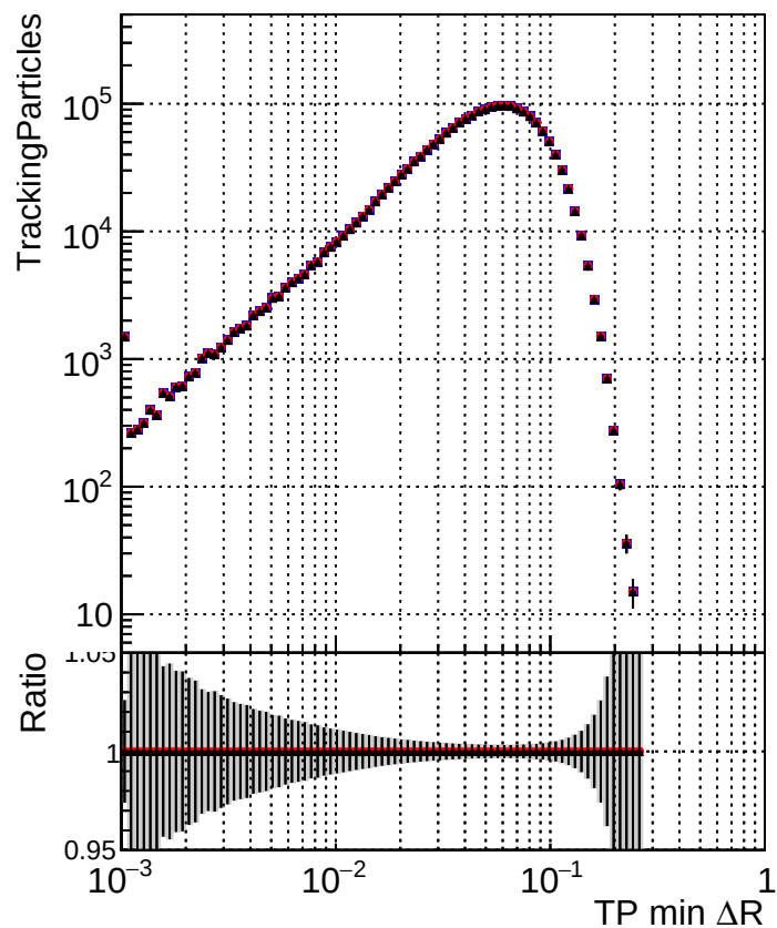
N of simulated tracks DQM_TT_original_lowpt DQM_TT_newbranch_lowpt_pLess DQM_TT_newbranch_lowpt_pLessMVA
