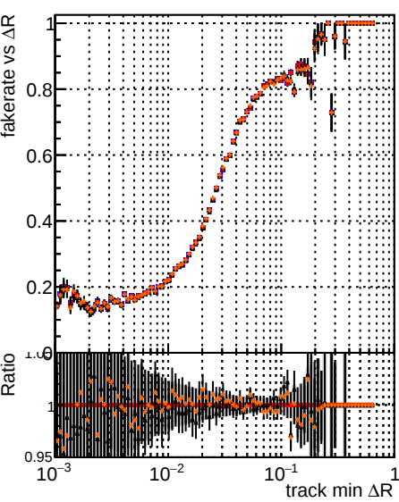
Fake rate vs \Delta R (track, jet) Legend: - original lowpt - newbranch lowpt - original lowpt pLess - newbranch lowpt pLess
