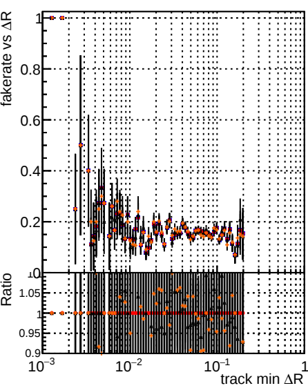
Fake rate vs \Delta R(\text{track, jet}) Legend: \Delta R(\text{track, jet}) (black dots) \Delta R(\text{track, jet}) (red dots) \Delta R(\text{track, jet}) (blue dots) \Delta R(\text{track, jet}) (orange dots) \Delta R(\text{track, jet}) (black dots) \Delta R(\text{track, jet}) (red dots) \Delta R(\text{track, jet}) (blue dots) \Delta R(\text{track, jet}) (orange dots)
