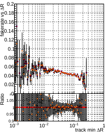
Fake rate vs \Delta R(\text{track}, \text{jet}) Legend: \square original lowpt, \square newbranch lowpt, \square original lowpt pless, \square newbranch lowpt pless
