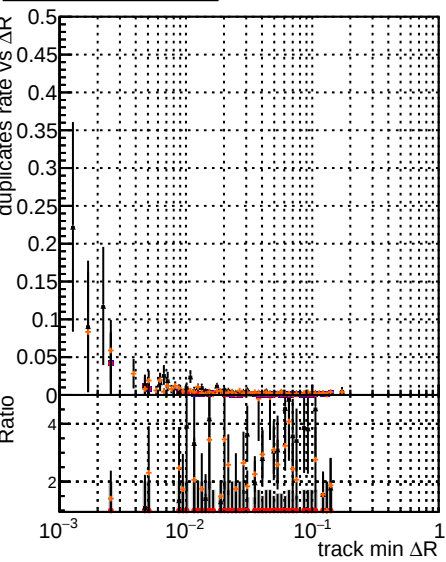
DOM TT original lowpt DOM TT newbranch lowpt DOM TT original lowpt pLess DOM TT newbranch lowpt pLess
