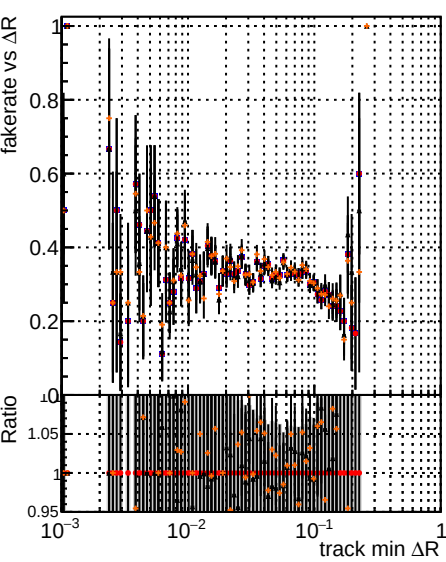
Fake rate vs \Delta R(\text{track, jet}) Legend: original lowpt (black line with dots) newbranch lowpt (red line with dots) original lowpt pless (black line with dots) newbranch lowpt pless (red line with dots)
