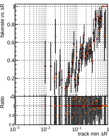
Fake rate vs \Delta R(\text{track, jet}) Legend: original lowpt (black square) newbranch lowpt (red circle) original lowpt pLess (black square) newbranch lowpt pLess (red circle)
