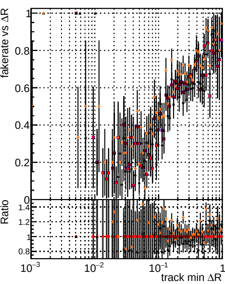
Fake rate vs \Delta R(\text{track, jet}) Legend: original lowpt (black line) newbranch lowpt (red line) original lowpt pless (orange line) newbranch lowpt pless (blue line)
