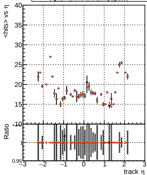
— DQM_TT_original_lowpt — DQM_TT_newbranch_lowpt — DQM_TT_original_lowpt_pLess — DQM_TT_newbranch_lowpt_pLess
