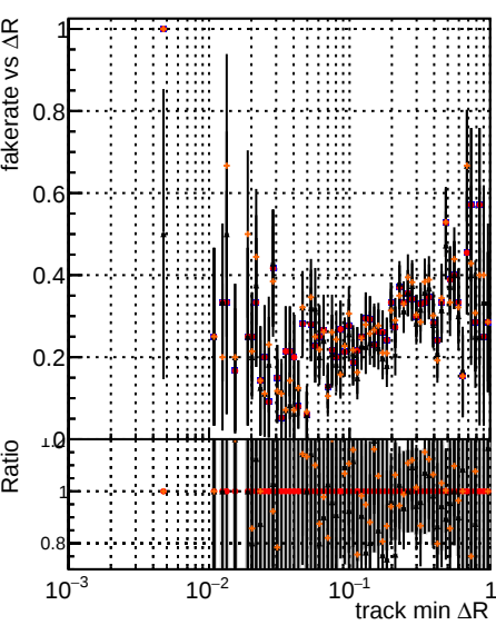
Fake rate vs \Delta R(\text{track, jet}) Legend: original lowpt (black) newbranch lowpt (blue) original lowpt pless (red) newbranch lowpt pless (orange)
