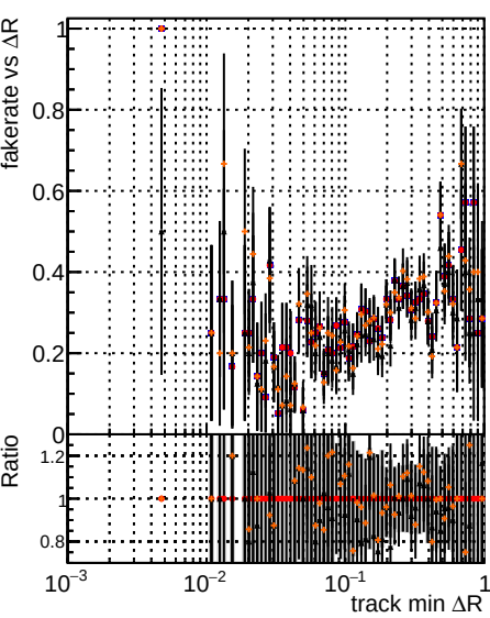
Fake rate vs \Delta R(\text{track, jet}) Legend: original lowpt (black line) newbranch lowpt (red line) original lowpt pless (blue line) newbranch lowpt pless (orange line)
