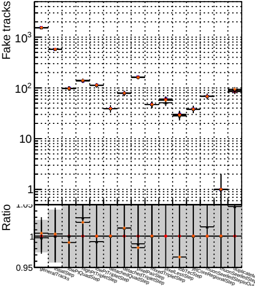
Number ■ DQM_TT_original_lowpt ● DQM_TT_newbranch_lowpt ▲ DQM_TT_original_lowpt_pLess ◆ DQM_TT_newbranch_lowpt_pLess
