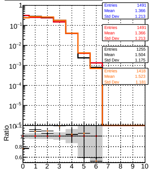
mean hit DQM_TT_original_lowpt DQM_TT_newbranch_lowpt DQM_TT_original_lowpt_pLess DQM_TT_newbranch_lowpt_pLess
