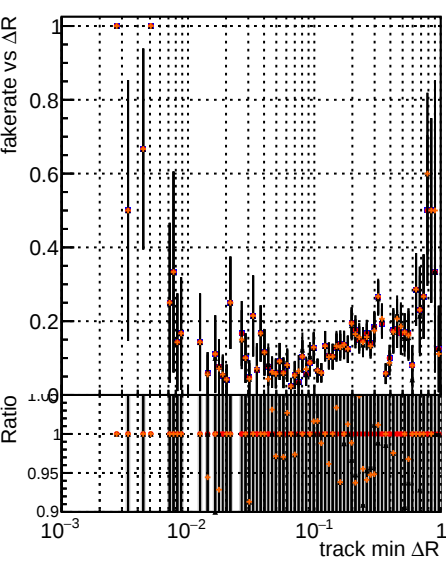
Fake rate vs \Delta R(\text{track, jet}) Legend: original lowpt (black line) newbranch lowpt (red line) original lowpt pLess (black line with dots) newbranch lowpt pLess (red line with dots)
