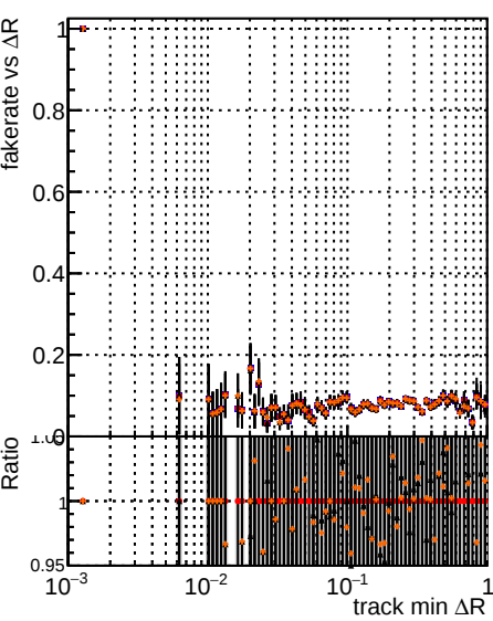
Fake rate vs \Delta R(\text{track, jet}) Legend: original lowpt (black squares) newbranch lowpt (red circles) original lowpt pLess (black squares) newbranch lowpt pLess (red circles)
