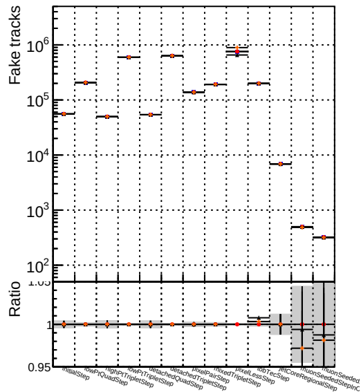
Number of tracks vs collection Legend: Blue line: DQM TT original lowpt Red line: DQM TT newbranch_lowpt Black line: DQM TT original_lowpt_pLess Orange line: DQM TT newbranch_lowpt_pLess
