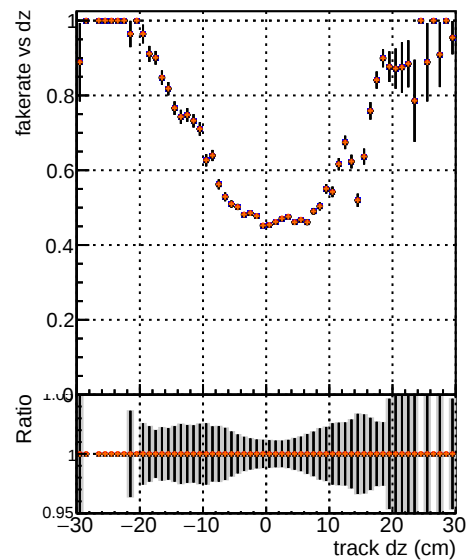
Fake rate vs d Legend: DGM TT original DGM TT newbranch DGM TT original lowpt DGM TT newbranch lowpt DGM TT original pLess
