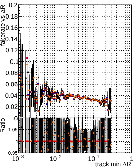
Fake rate vs \Delta R(\text{track}, \text{jet}) Legend: original lowpt newbranch lowpt original lowpt pless newbranch lowpt pless
