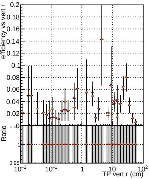
Efficiency vs TP vert r (cm) DOM TT original_lowpt DOM TT newbranch_lowpt DOM TT original_lowpt_pLess DOM TT newbranch_lowpt_pLess
