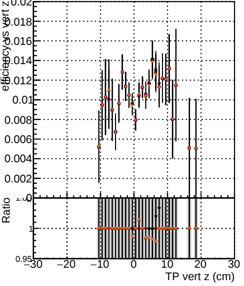
Efficiency vs TP vert z (cm) DOM TT original_lowpt DOM TT newbranch_lowpt DOM TT original_lowpt_pLess DOM TT newbranch_lowpt_pLess
