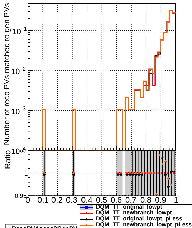
RecoPVAssoc2GenPVMatched_missing
