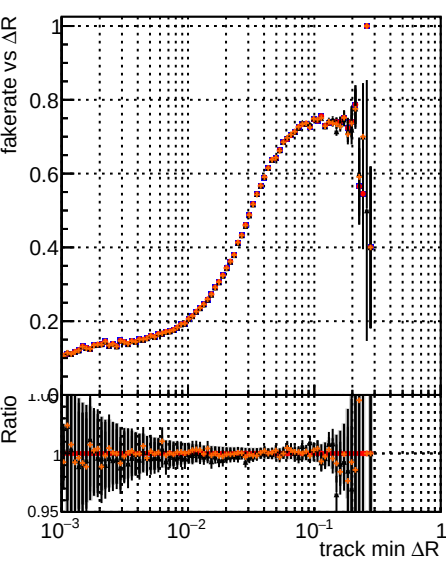
Fake rate vs \Delta R (track, jet) Legend: original lowpt (black dots), newbranch lowpt (red dots), original lowpt pLess (black dots), newbranch lowpt pLess (red dots)
