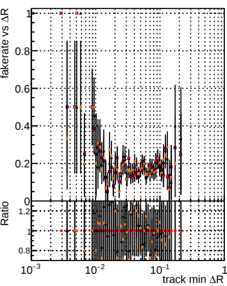
Fake rate vs \Delta R(\text{track, jet}) Legend: DOM TT original lowpt DOM TT newbranch lowpt DOM TT original lowpt pLess DOM TT newbranch lowpt pLess
