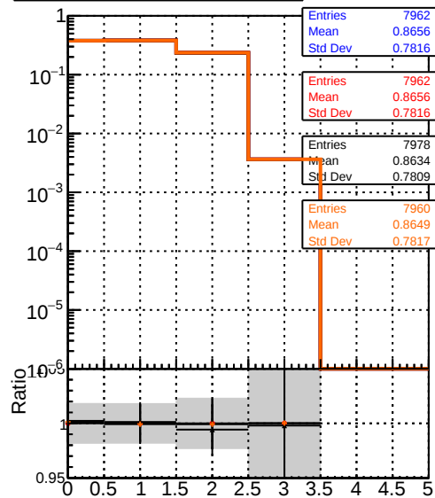
mean hits DQM_TT_original_lowpT DQM_TT_newbranch_lowpT DQM_TT_original_lowpT_pLess DQM_TT_newbranch_lowpT_pLess
