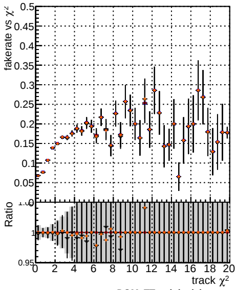
Fake rate vs. - DOM - original_lowpt - DOM - newbranch_lowpt - DOM - newbranch_lowpt_plus
