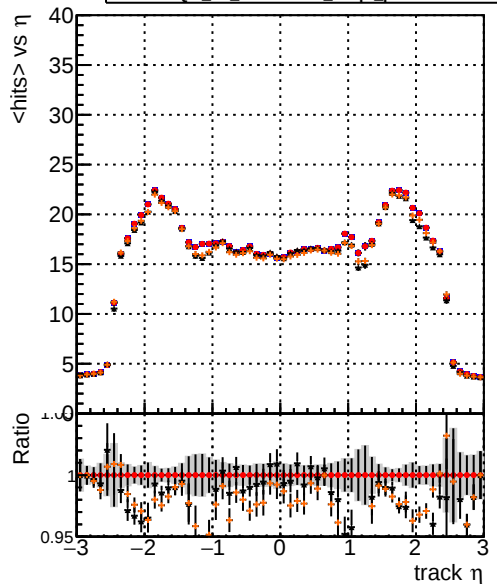
mean hits vs \eta — DQM_TT_original_lowpt — DQM_TT_newbranch_lowpt — DQM_TT_original_lowpt_pLess — DQM_TT_newbranch_lowpt_pLess
