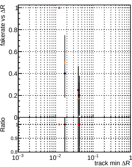
Fake rate vs ΔR(track, jet) Legend: original_lowpt (black line) newbranch_lowpt (blue line) original_lowpt_pless (red line) newbranch_lowpt_pless (orange line)
