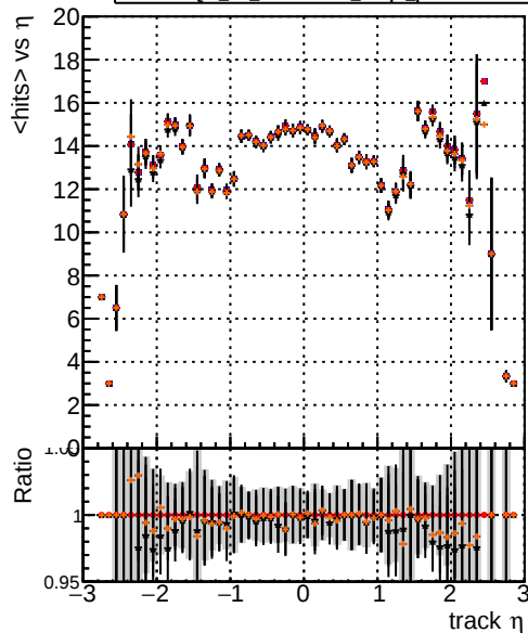
— DQM_TT_original_lowpt — DQM_TT_newbranch_lowpt — DQM_TT_original_lowpt_pLess — DQM_TT_newbranch_lowpt_pLess mean hits
