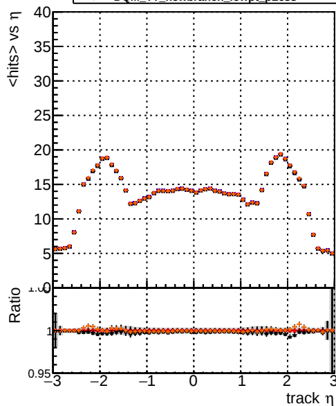
— DQM_TT_original_lowpt — DQM_TT_newbranch_lowpt — DQM_TT_original_lowpt_pLess — DQM_TT_newbranch_lowpt_pLess mean hit
