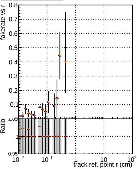
Fake rate vs verpos Legend: DOM TT original lowpt, DOM TT newbranch lowpt, DOM TT original lowpt pless, DOM TT newbranch lowpt pless
