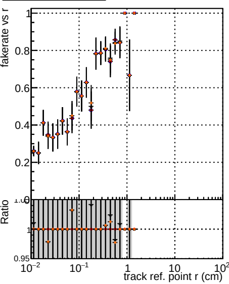
Fake rate vs v Legend: original lowpt (black line with dots) newbranch lowpt (red line with dots) original lowpt pless (orange line with dots) newbranch lowpt pless (blue line with dots)
