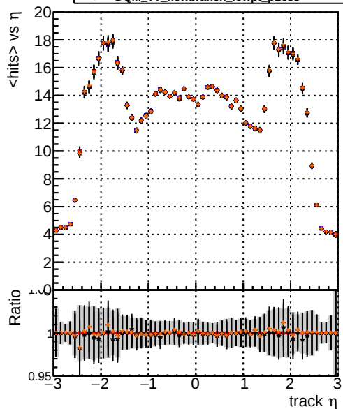
mean hit DQM_TT_original_lowpt DQM_TT_newbranch_lowpt DQM_TT_original_lowpt_pLess DQM_TT_newbranch_lowpt_pLess
