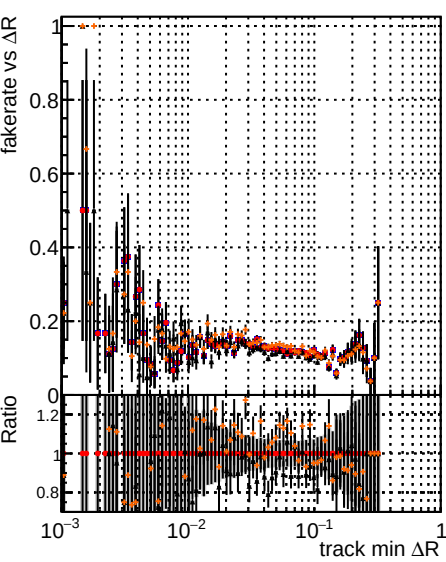
Fake rate vs \Delta R (track, jet) Legend: original lowpt (black) newbranch lowpt (red) original lowpt pless (grey) newbranch lowpt pless (orange)
